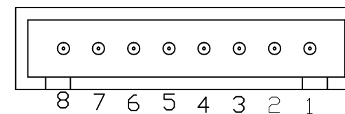
K1(scale 4:1): 8Pin pitch=2.50mm Part No: SYUIN 8824-08
