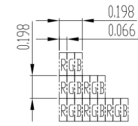
Pixel Details SCALE=30/1
