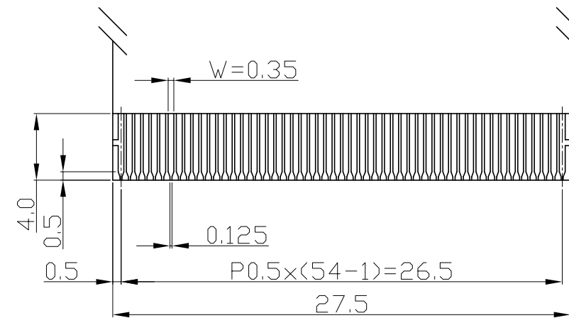
LCD FPC Details (Conductor side) Scale=3/1
