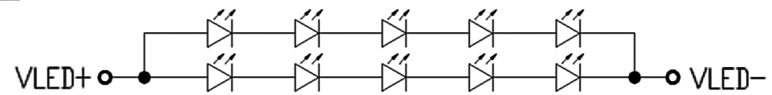
CIRCUIT DIAGRAM
