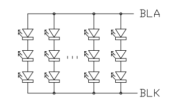
Backlight Circuit (No. of LEDs = 3x10pcs) Scale=free
