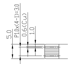
Touch Panel FPC Terminals Details (Conductor Side) Scale=free
