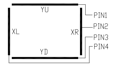
Touch Panel Logic Details Scale=free
