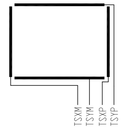
Touch Panel Logic Details Scale=free
