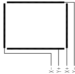
Touch Panel Logic Details Scale=free
